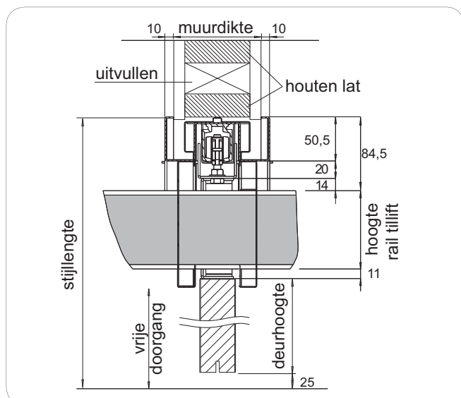
verticale doorsnede Silence Ultra Care
