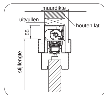
verticale doorsnede SIW Electric
